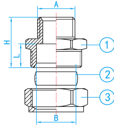
SECTION VIEW
