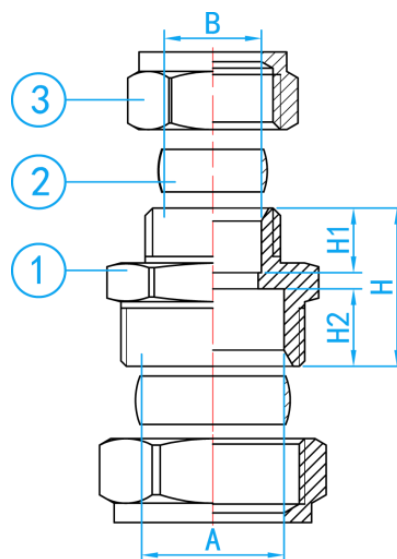
SECTION VIEW
