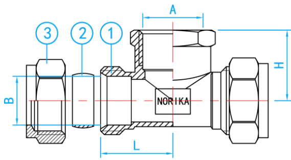
SECTION VIEW
