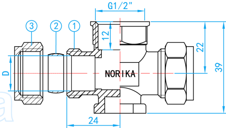
SECTION VIEW
