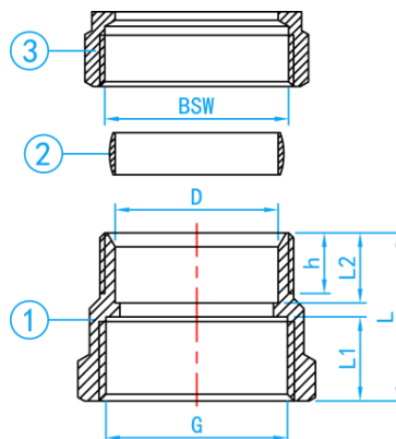
SECTION VIEW
