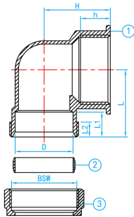
SECTION VIEW
