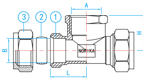
SECTION VIEW
