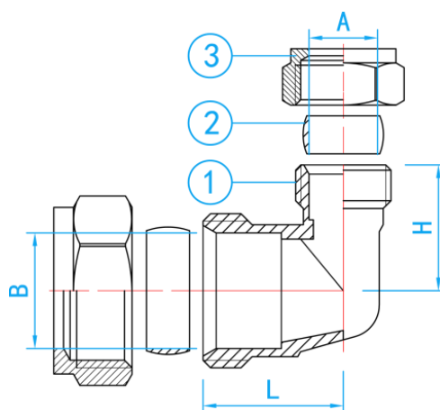
SECTION VIEW
