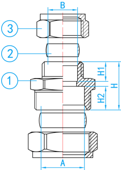
SECTION VIEW
