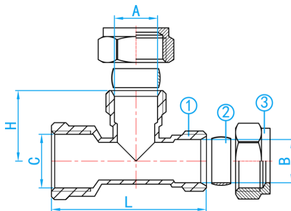
SECTION VIEW
