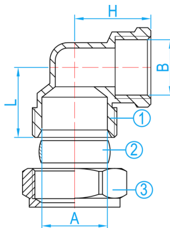
SECTION VIEW
