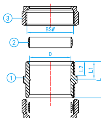
SECTION VIEW
