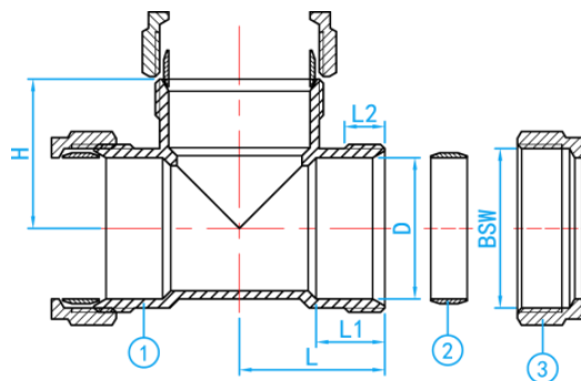
SECTION VIEW
