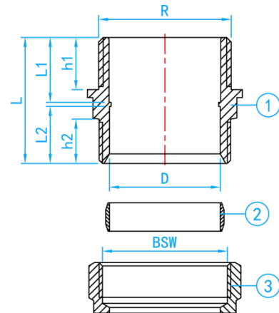
SECTION VIEW
