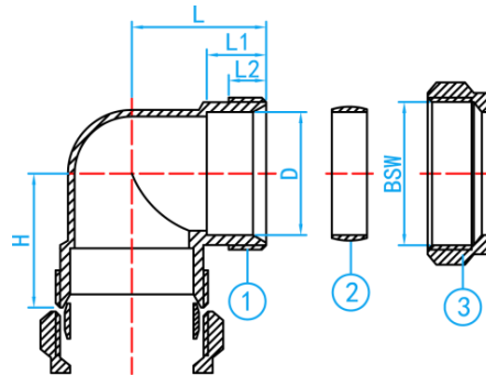
SECTION VIEW
