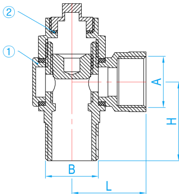
SECTION VIEW
