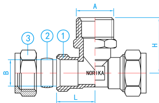
SECTION VIEW
