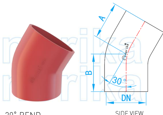
30° BEND
