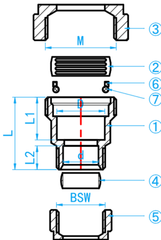
SECTION VIEW
