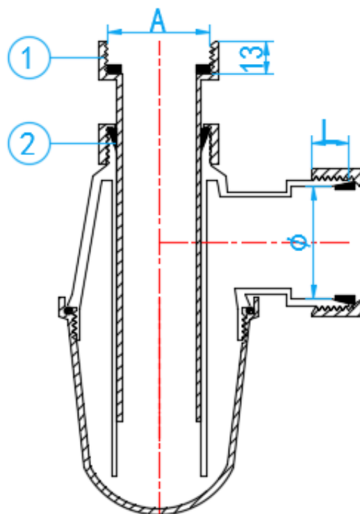
SECTION VIEW
