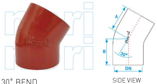
30° BEND
