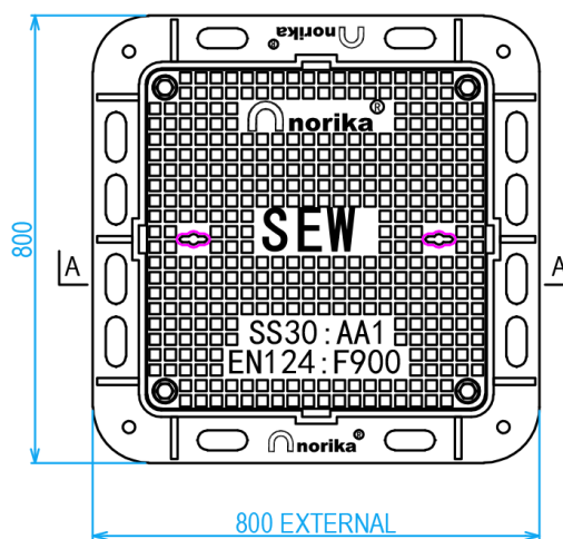
HALF COVER REMOVED TOP VIEW
