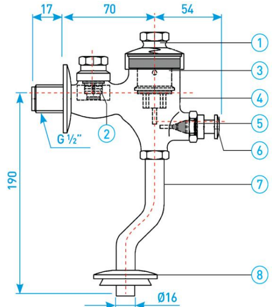
SIDE-CROSS SECTION VIEW
