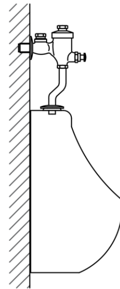
INSTALLATION ASSEMBLY
