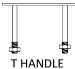
T HANDLE
