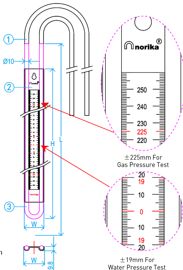
SIDE VIEW
