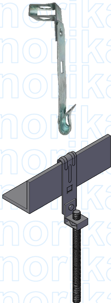
INSTALLATION ASSEMBLY
