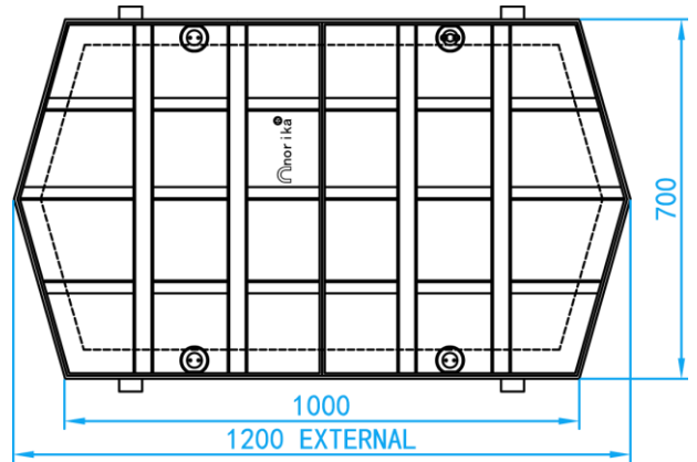
RECESSED MOSAIC TILING SIDE
