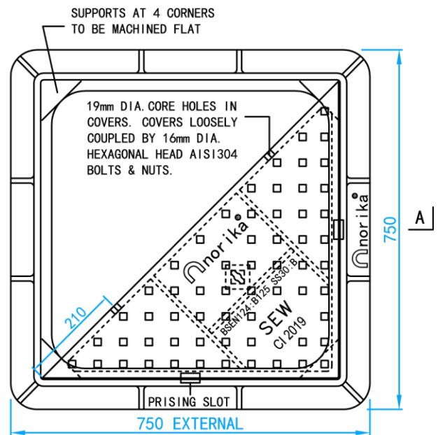
HALF COVER REMOVED TOP VIEW
