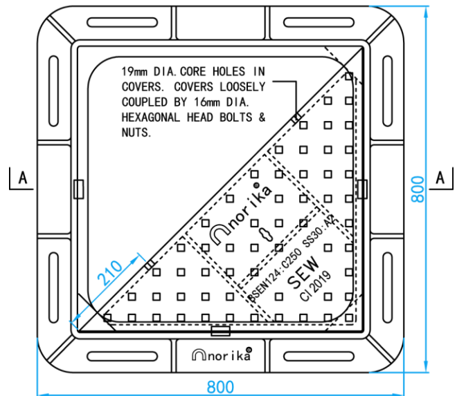
HALF COVER REMOVED TOP VIEW
