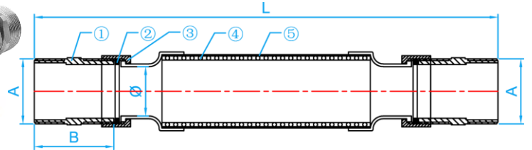
SECTION VIEW
