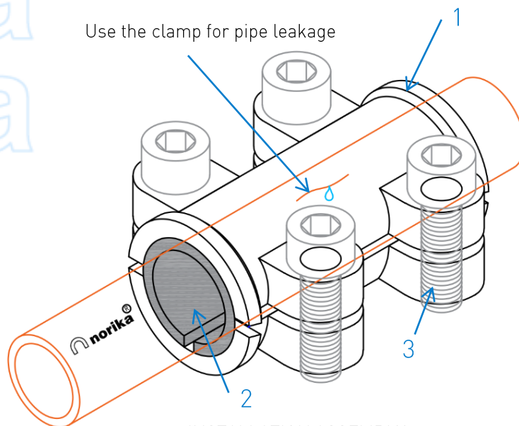
INSTALLATION ASSEMBLY
