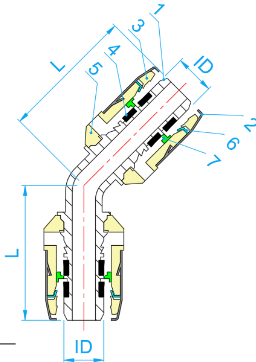
SECTION VIEW
