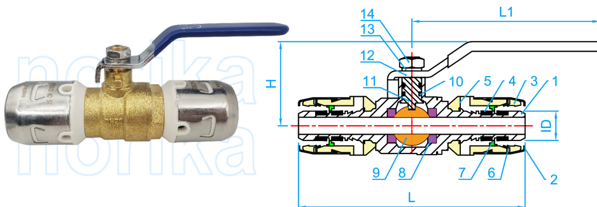
SECTION VIEW
