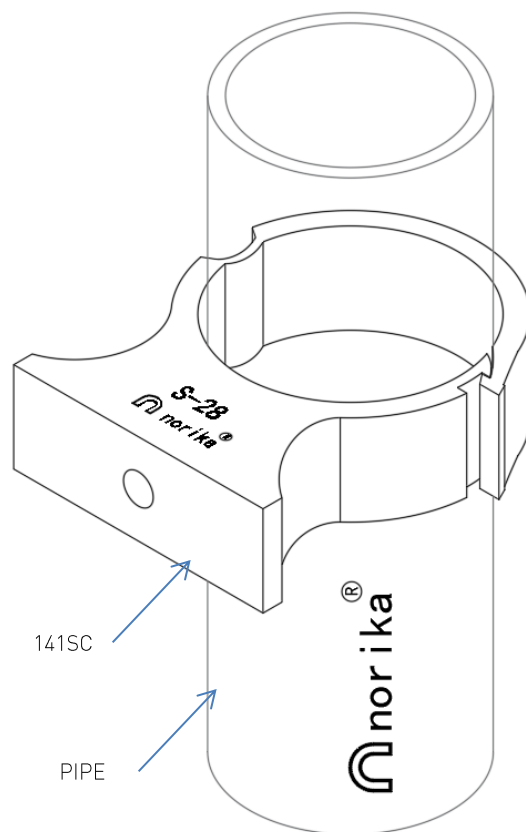
INSTALLATION ASSEMBLY
