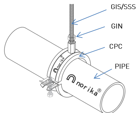
INSTALLATION ASSEMBLY
