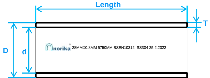
CROSS SECTION VIEW
