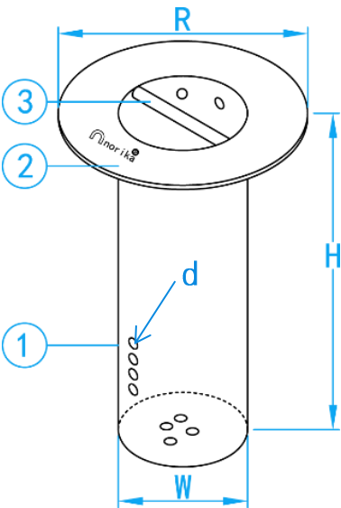
3-D VIEW
