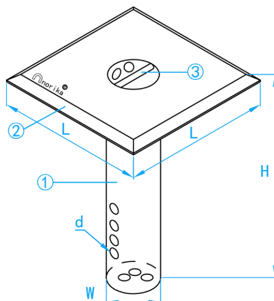
3-D VIEW
